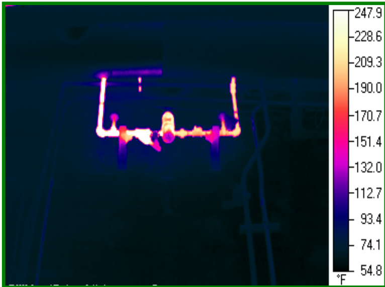
Excessive steam trap leak on Unit # 4190
