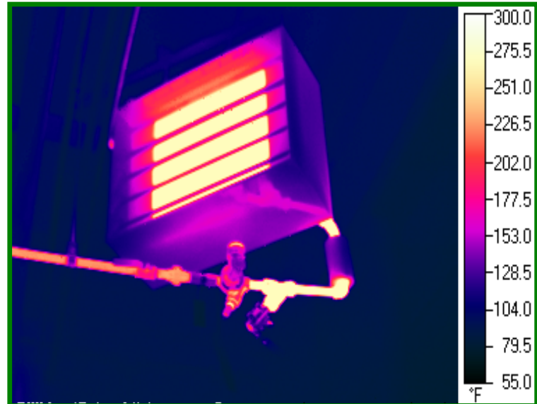
Steam Trap Samples show proper operation.
